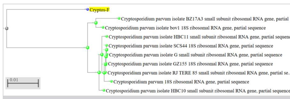
Figure 5. Phylogenetic tree generated using the BLAST distance-tree method based on pairwise sequence alignments of the SSU-rRNA gene. The sequence obtained in this study (Crypto-F / Query_3448041) clustered closely with Cryptosporidium parvum isolates, confirming its identity as C. parvum .
