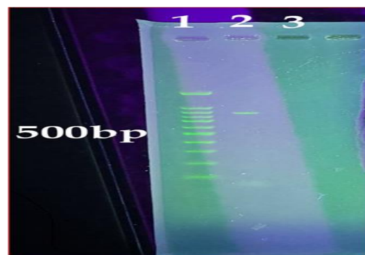
Figure 2. Agarose gel electrophoresis (1% agarose, ethidium bromide staining) of the PCR products amplified from the ITS1-rRNA gene. Lane L: 100 bp DNA ladder; Lane 1: positive control ( Cryptosporidium parvum ) ; Lane 2: PCR-positive water sample; Lane 3: negative sample.
